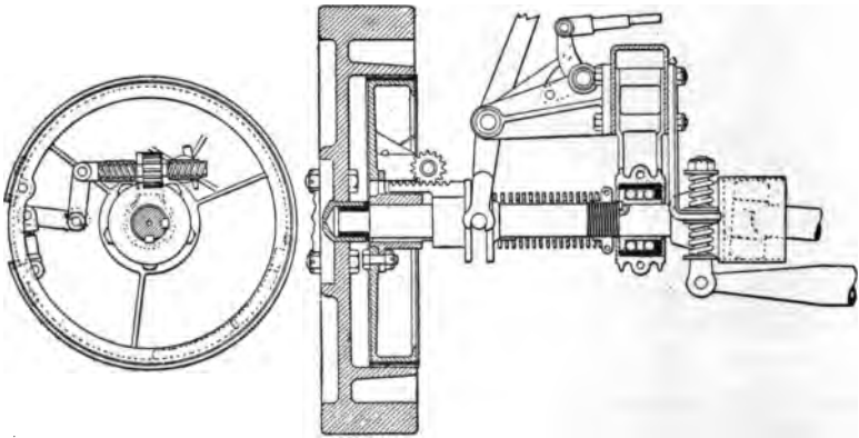
FIG. 243.—End View and Cross Section of the Packard Expanding Ring Clutch.
